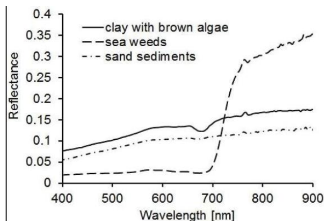
Figure 11-Spectral signatures of different sediment types in intertidal flats, Wadden Sea. Reference: Dube, 2012 (Figure 4-1, page 15).
