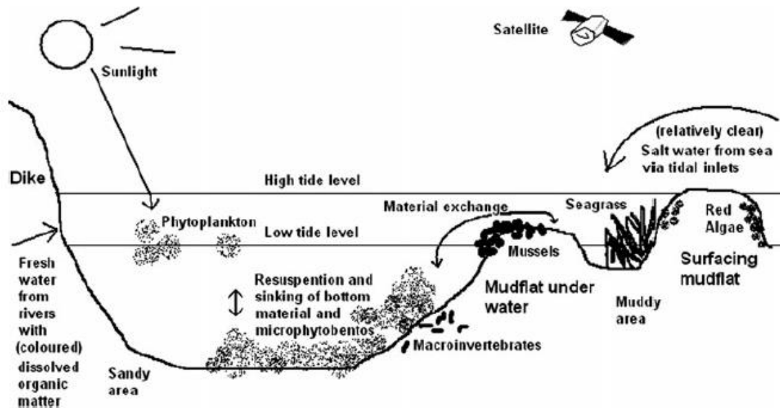
Figure 8- Schematic overview of substances and occurrence of processes in the Wadden Sea. (Reference: Hommersom et al (2010) (Figure 3, page 88)).
