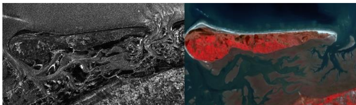
Figure 2-Radar ERS SAR image, date 20 August 2010 (left), multi-spectral DEIMOS image, date April 14, 2010 (right). The radar image has one band (intensity image) whereas the multi-spectral image is presented in a combination of 3 bands (near-infrared, red and green).
