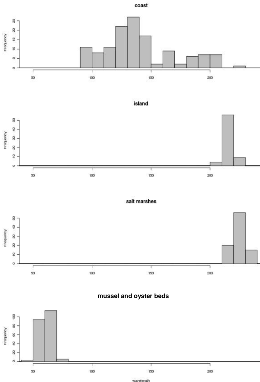
Figure 12- Spectral difference between coast (coastal land); island (main land of Ameland), salt marshes and mussel and oyster beds, band 2- Green on Worldview-2 image, resolution 2.5 meters. Date of acquisition- July 21, 2006.
