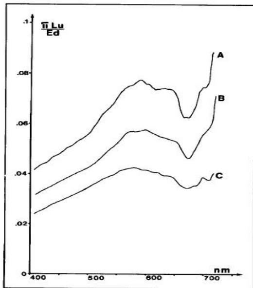
Figure 10-Reflectance of very dry sand (A), wet sand (B) and fine-grained mud (C) on Landsat image, resolution 30 meters. Reference: Bartholdy and Folving, 1986 (Figure 6, page 341).
