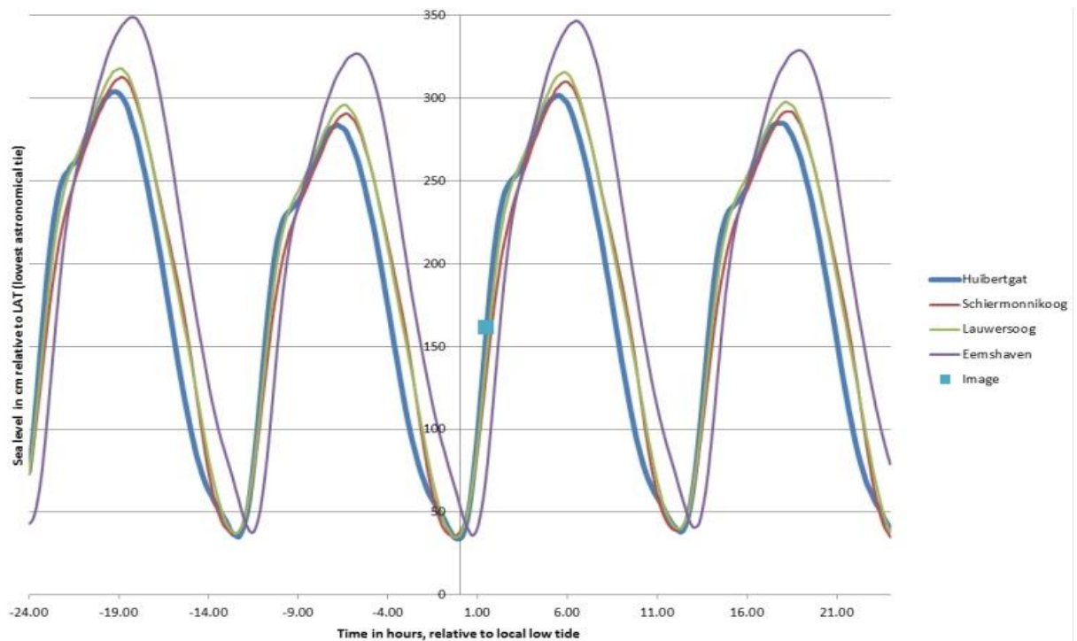
Figure 3-Tidal movements over the stations of Huibertgat (H), Schiermonnikoog (S), Eemshaven (E). Reference: Davaasuren, Stapel et al (2012).
