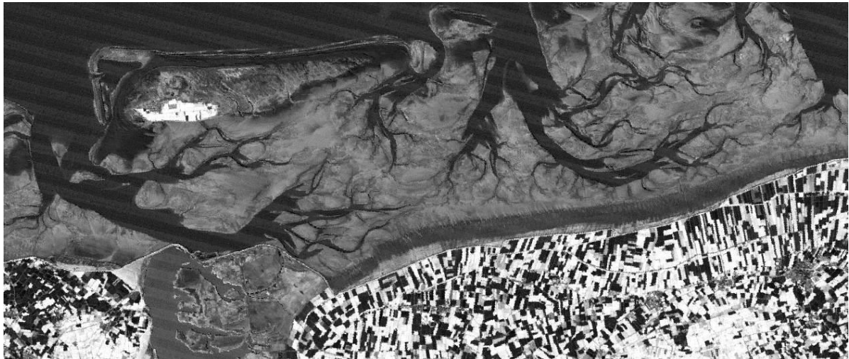
Figure 14-Soil moisture index. Image Landsat-5, date of acquisition 25 November, 1995.
