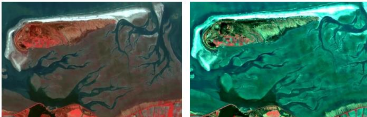
Figure 7-Uncorrected (left) and atmospheric corrected image (right). The corrected image is enhanced in green band. Image- DEIMOS-2, date of acquisition March 15, 2012.
