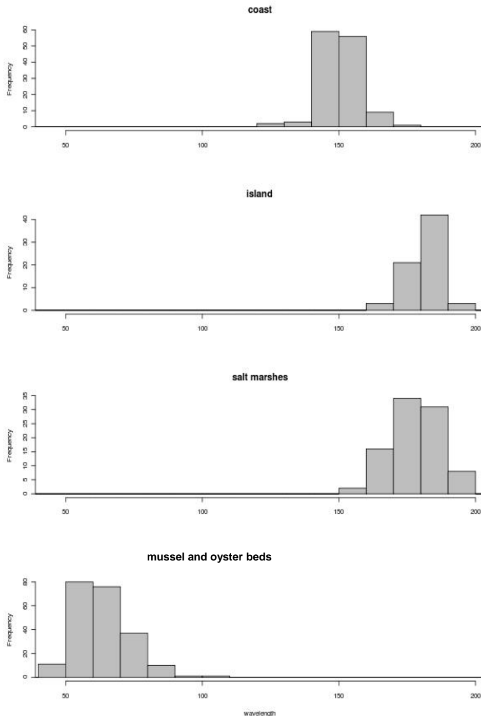
Figure 13-Spectral difference between coast (coastal land); island (main land of Ameland), salt marshes and mussel and oyster beds, band 3- Red on Worldview-2 image, resolution 2.5 meters. Date of acquisition- July 21, 2006.
