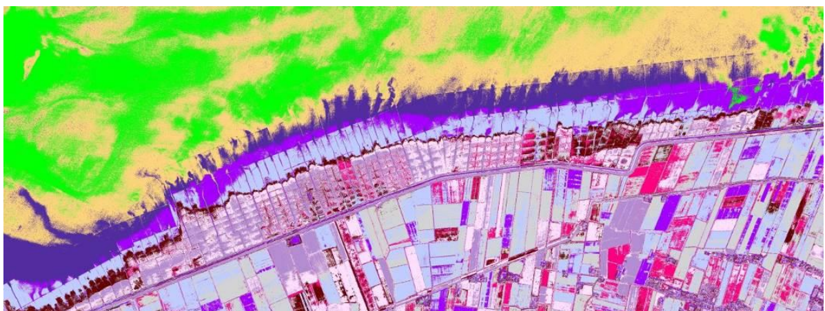
Figure 15-Soil indexing, north-east of Groningen, De Marne. Soil with high moisture content in violet color, dry soil areas in red and pink. Deep water areas in green, shallow water in yellow. Worldview-2 image acquired on September 26, 2011.
