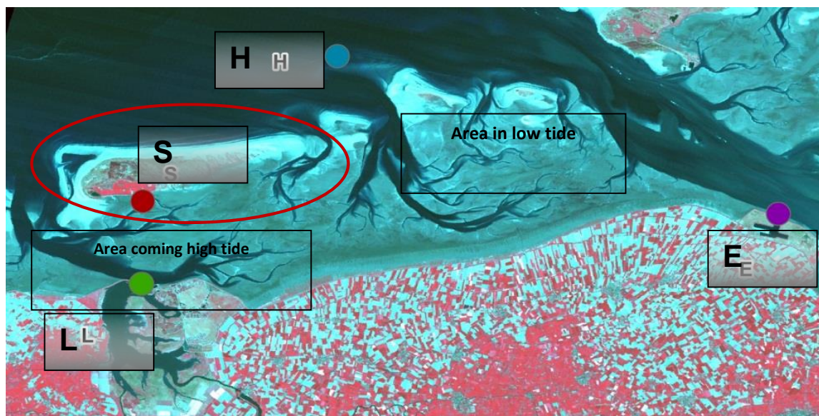
Figure 2-Landsat -5 Thematic Mapper image showing the tidal difference. Tide stations- Huibertgat (H), Lauwersoog (L), Schiermonnikoog (S) and Eemshaven (E).
