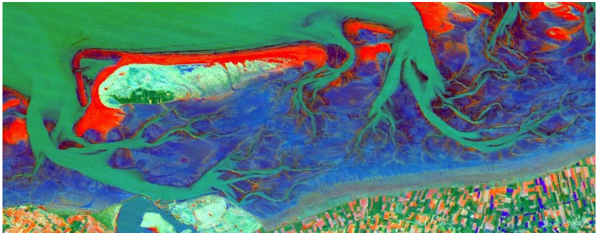
Figure 16-Vegetation indexing on Landsat-5 data using Near-infrared and red bands. Image date 25 November 1995.
