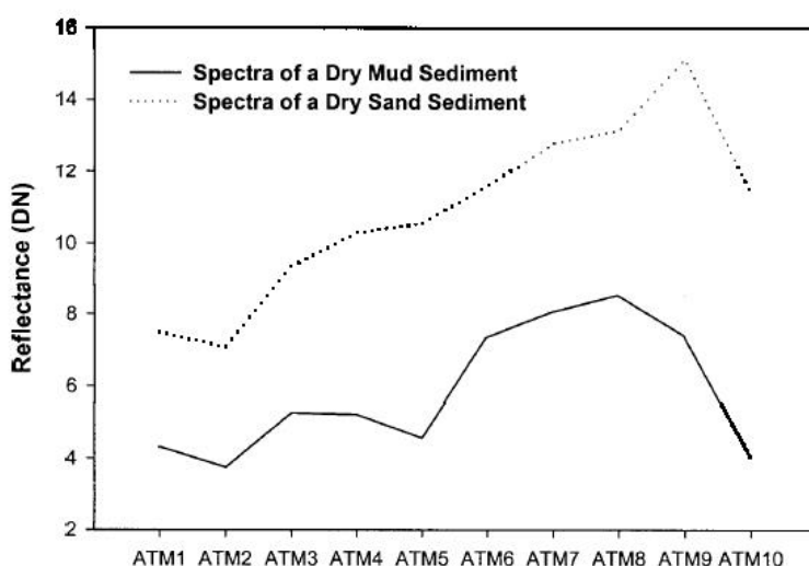
Figure 9-Difference in spectral signatures (spectra) between dry mud and dry sand sediment. Reference: Rainey et al 2000 (Figure 4, page 11).
