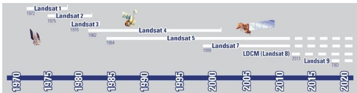
Figure 4- Landsat missions (U.S. Geological Survey, 2013).
