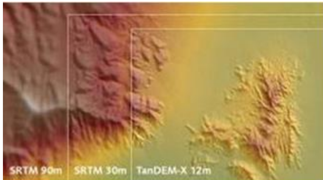
Figure 6-Comparison of global DEMs. SRTM in 90 meters, SRTM in 30 meters and TanDEM-X in 12 meters. (Source: Astrium GEO-Information Services, 2013. http://www.astrium-geo.com/worlddem )
